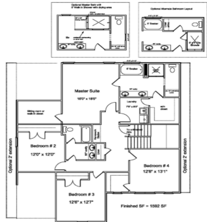
2 nd Floor Plan - The Merrill Park
