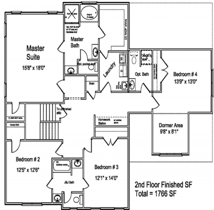
Pinehurst II 2nd Floor Plan
